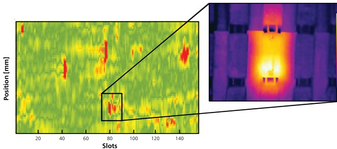
Figure 4. Comparison between a stray flux measurement of an entire stator and a section during a rated flux test on an old, decommissioned stator. The red areas indicate spots with fault currents higher than 100 mA measured during the stray flux measurement.
