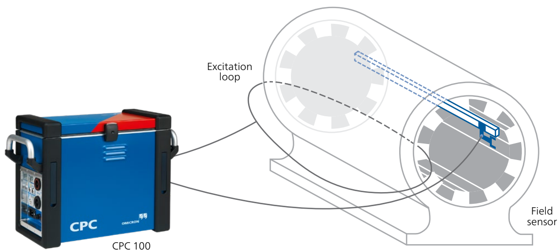
Figure 3. Test setup for a stator core imperfection detection test
