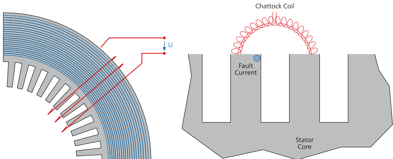
Figure 2: Left: Auxiliary winding and flux distribution within the stator core. Right: Faults are detected by a higher stray flux which is measured with a Chattock coil.
