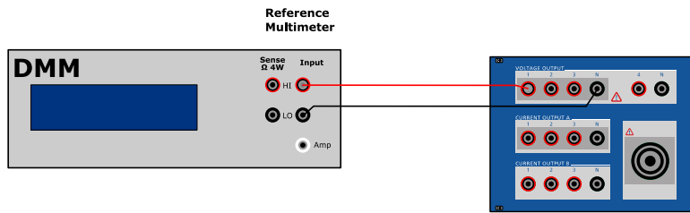
Figure 3 Voltage output setup
