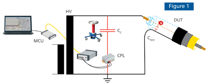
Typical PD measurement setup according to IEC 60270
