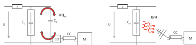
IEC compliant PD measurement
