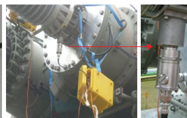
Example of using bushing tap adapters
