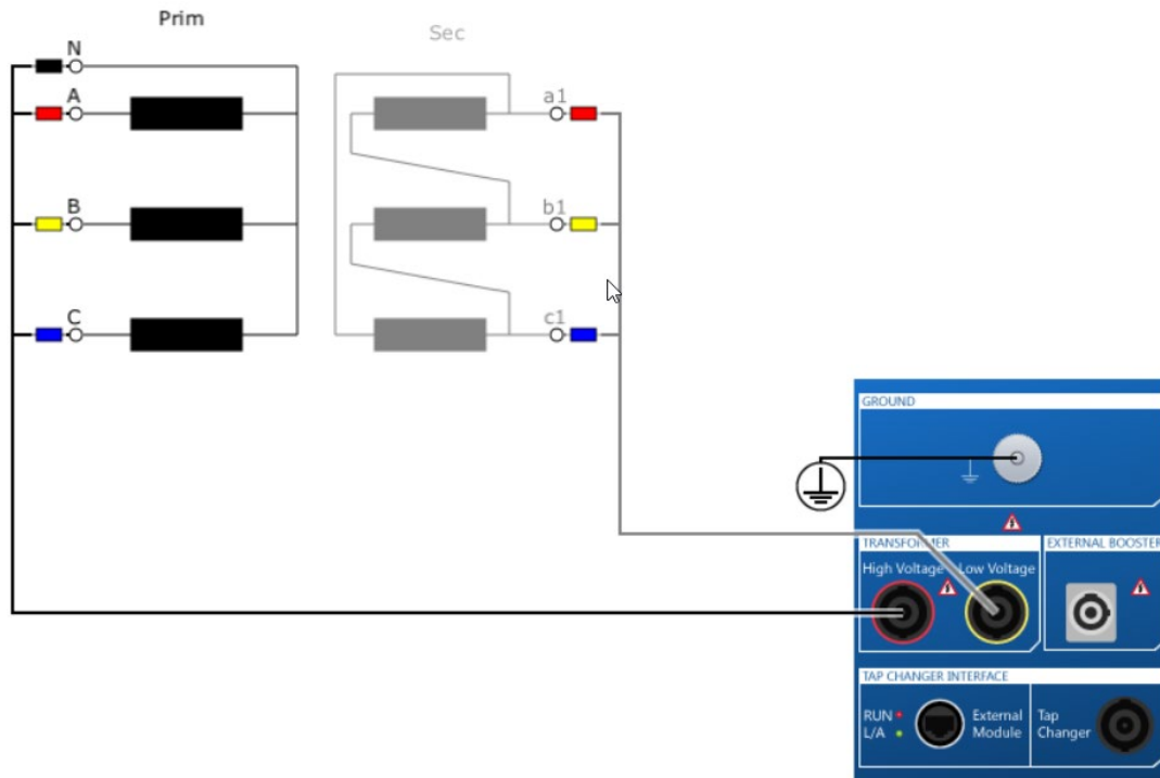
Figure 2: Typical connection set-up for a Star-Delta transformer using TESTRANO 600
