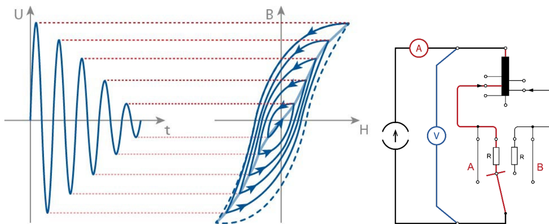
Figure 1: Demagnetizing the transformer core with sinusoidal signal
