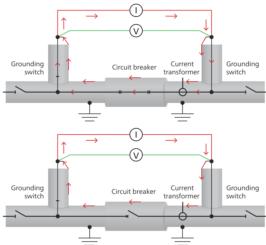
Contact resistance measurement with breaker closed (top) and with breaker open (bottom)
