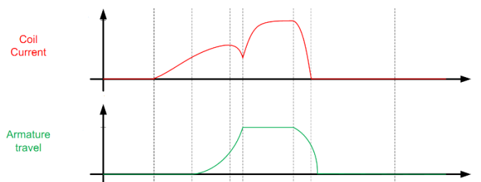
Figure 5 – Command Coil Current vs. Plunger Movement
