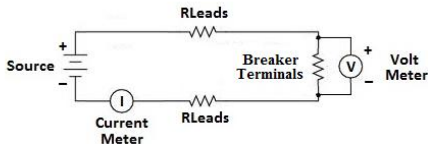
Figure 7 - Kelvin Connection Used for Contact Resistance Measurement
