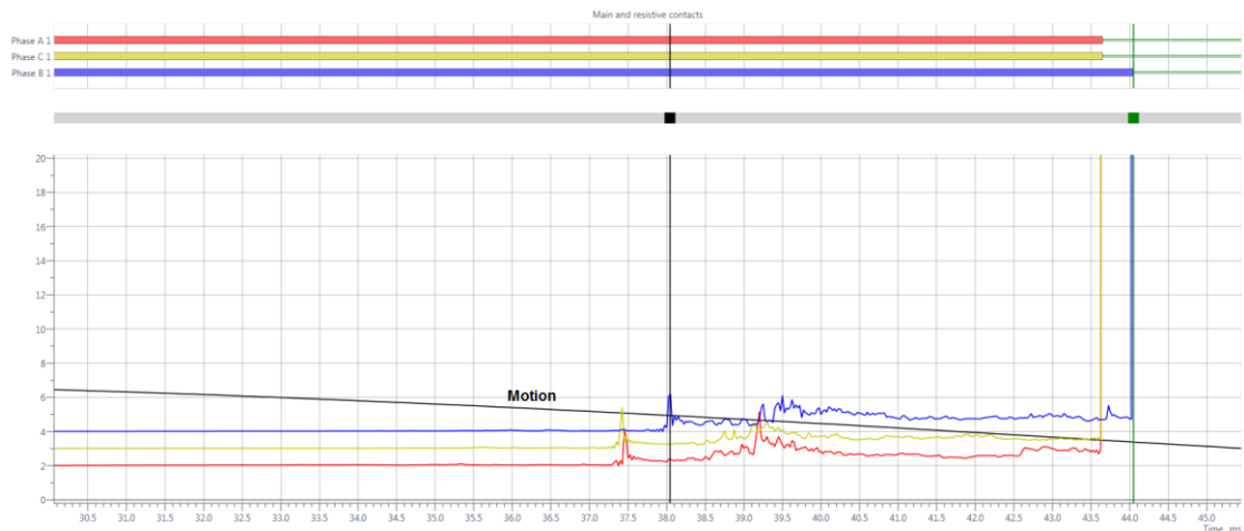
Figure 8 - Typical Dynamic Resistance Measurement
