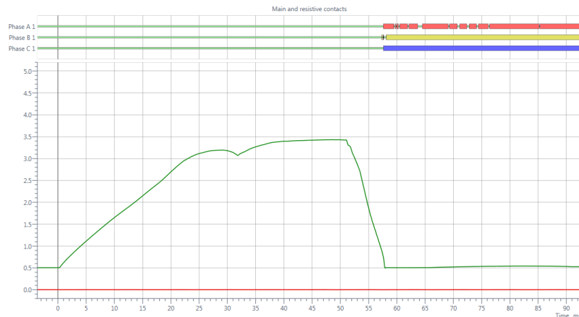
Figure 4 – Unusual Contact Bouncing
