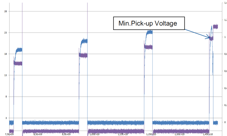
Figure 9 - Minimum Pick: Voltage and Current Responses
