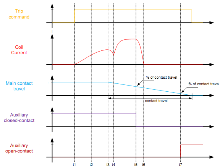
Figure 3 - Trip Operation Signals
