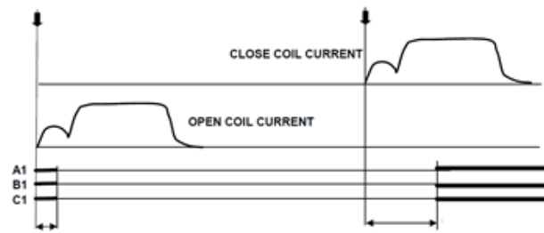
Figure 2 - Command Coil Currents and Main Contact State
