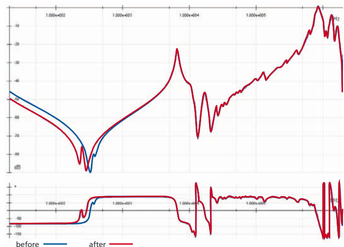
FRA measurement on phase W before and after demagnetization of the iron core.
