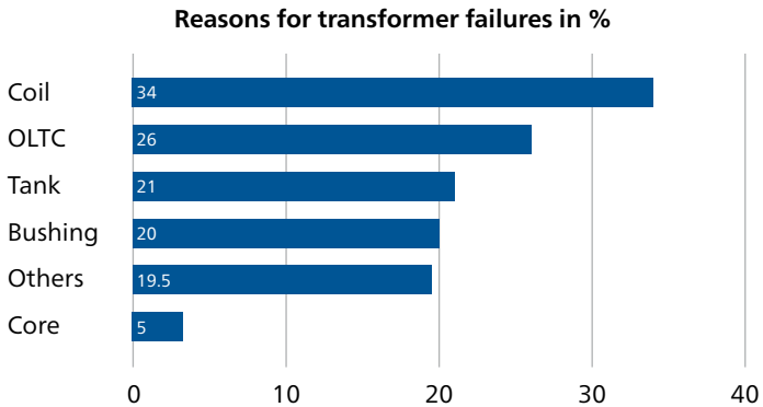
Transformer failure statistics (Viereck, Hillinger, Transform 2011)
