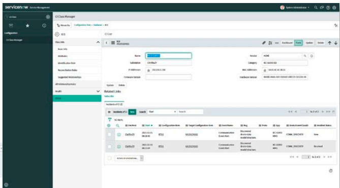
ServiceNow integration
