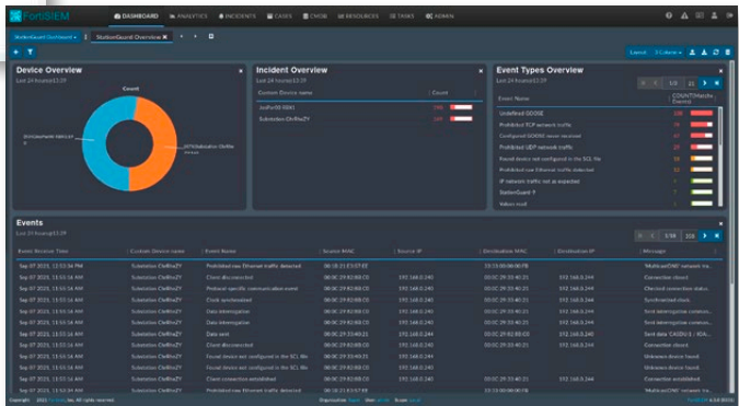
FortiSIEM integration
