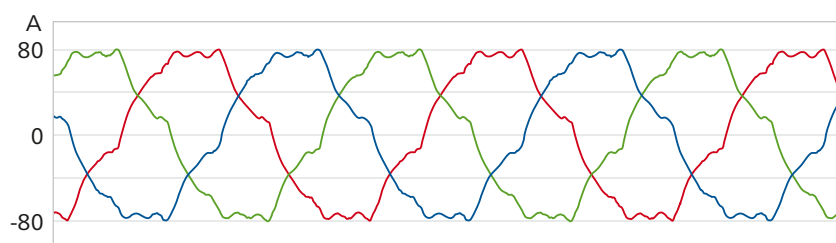
Figure 1: The acquired current waveforms show significant distortion, even at normal levels of solar radiation.
