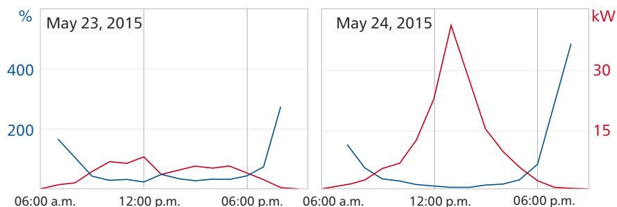
Figure 2: The THD_i reacted inversely proportional to the output.
