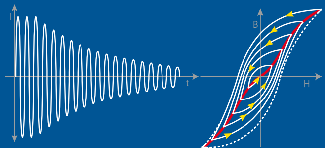
Demagnetization principle of iron cores
