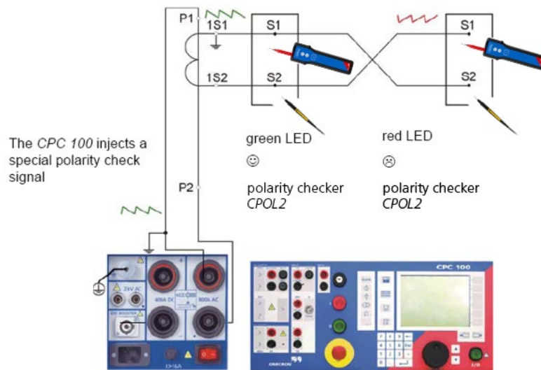
Fig. 6: Wiring testing with the CPOL2
