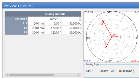
Fig. 1: Asymmetric injection with the QuickCMC
