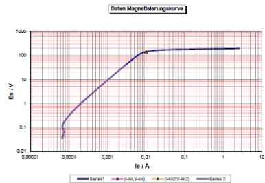
Fig. 4: Example of a test report
