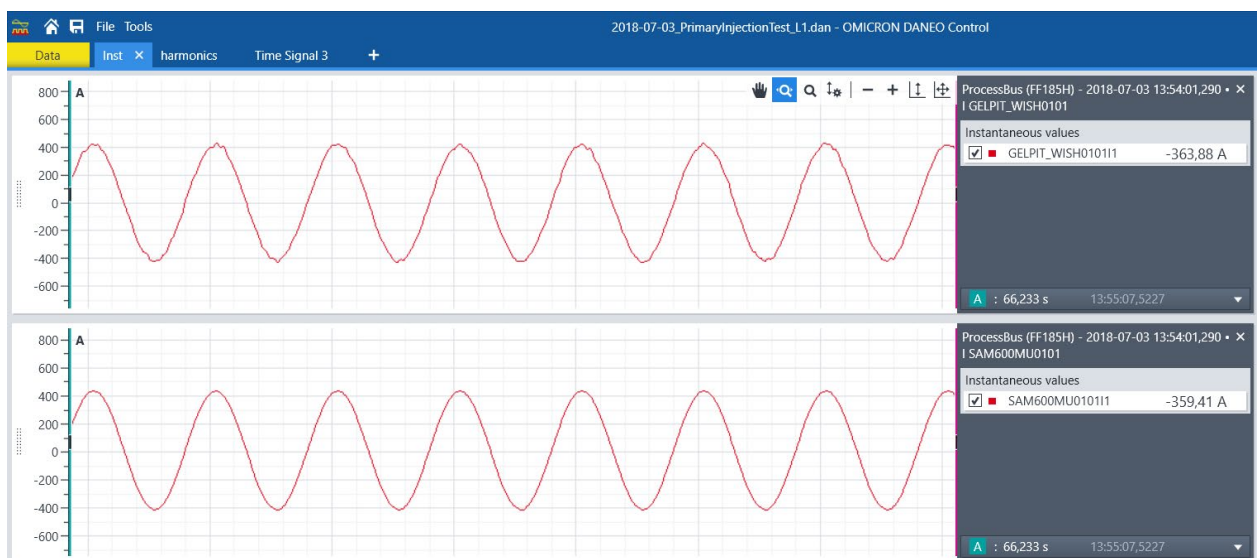
Fig. 8: Signal plot comparison using OMICRON's DANE0 400
