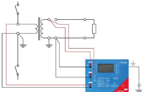
Fig. 3: Connection diagram for transformer measurement
