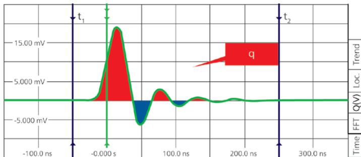
Measured Pulse – Typical classification of partial discharge sources
