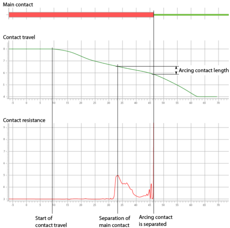
Figure 5: DRM curve interpretation for an SF6 circuit breaker
