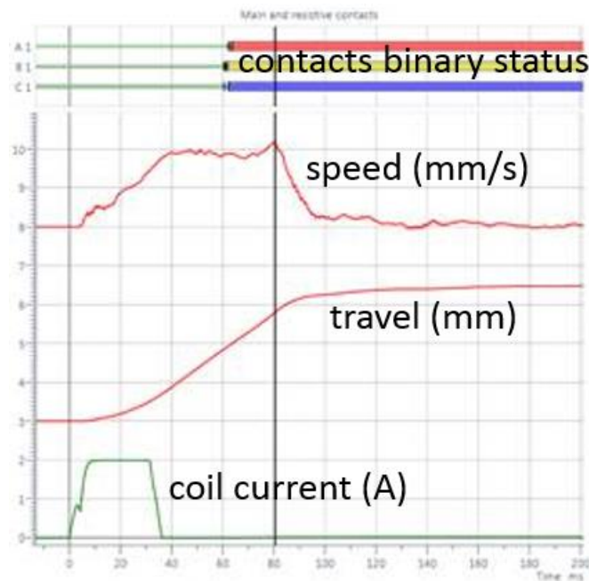
Figure 4: Damping analysis over time
