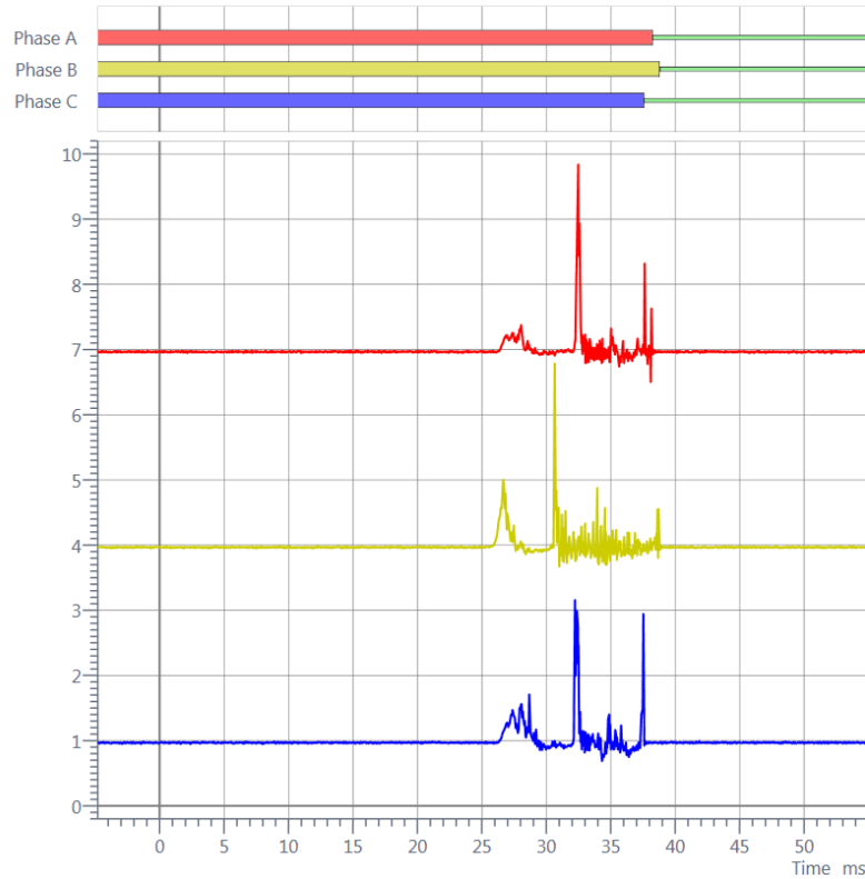
Figure 7: Current variations (A/s) over time through each phase during open operation of a 145 kV GIS circuit breaker
