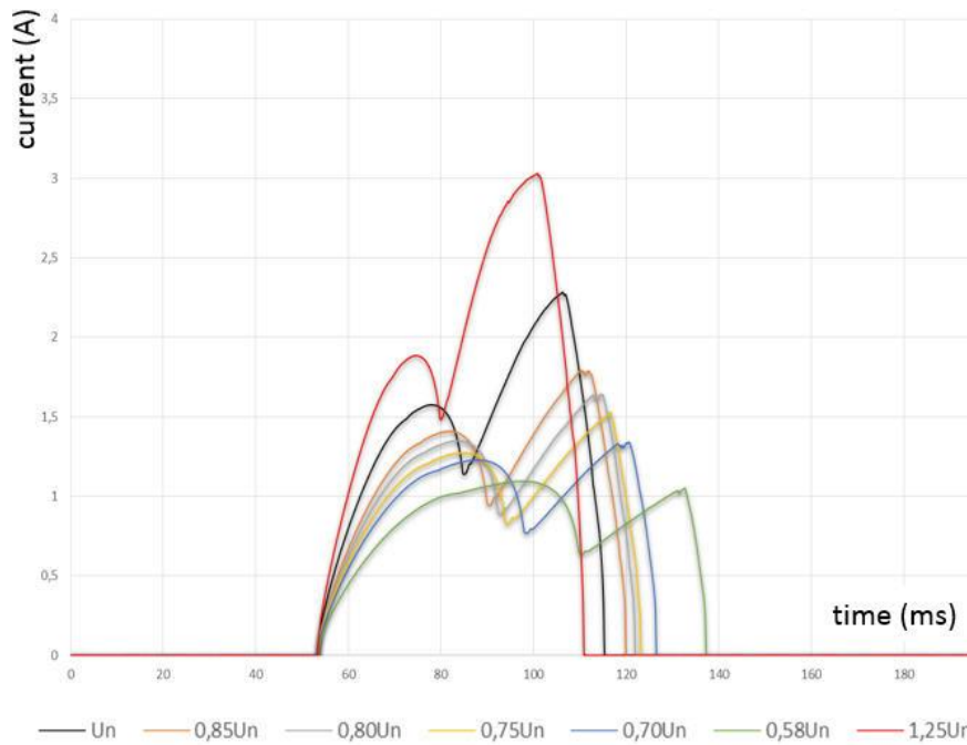
Figure 2: Coil current profile for different voltage from 0.25% to 1.25% of nominal voltage [3]
