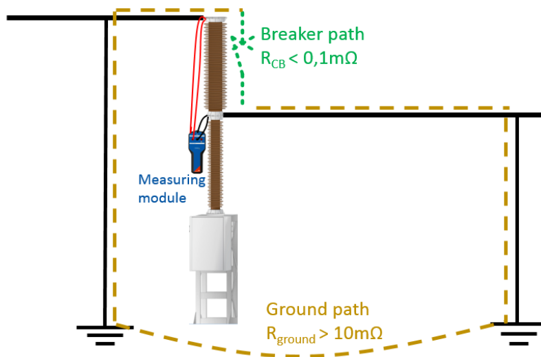
Figure 8: Testing DRM with both sides grounded
