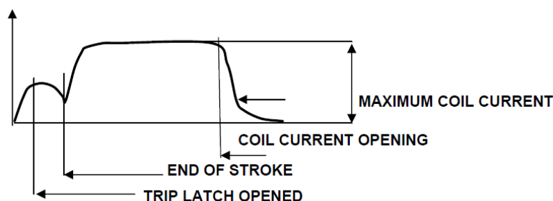
Figure 1: Typical coil current shape
