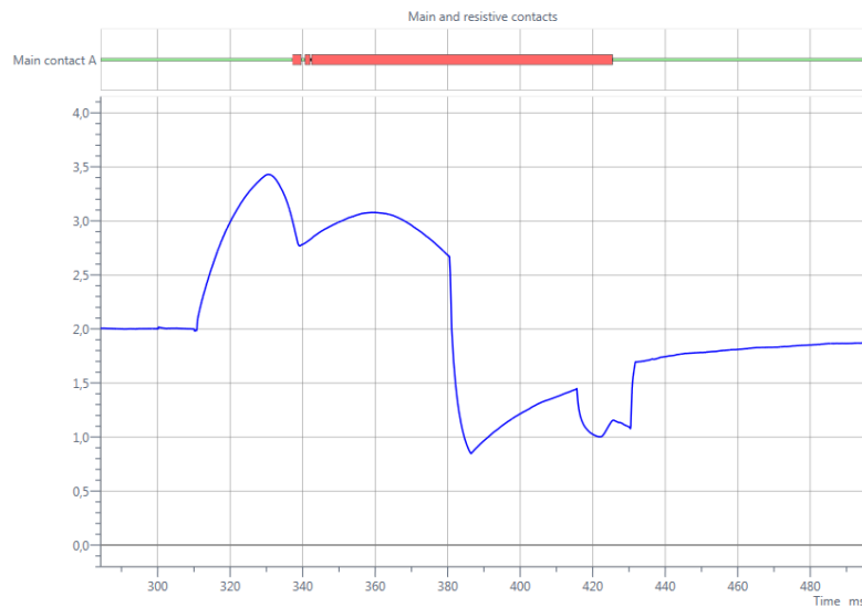
Figure 3: Actuating coil current over time in a CO sequence for a 2kV breaker
