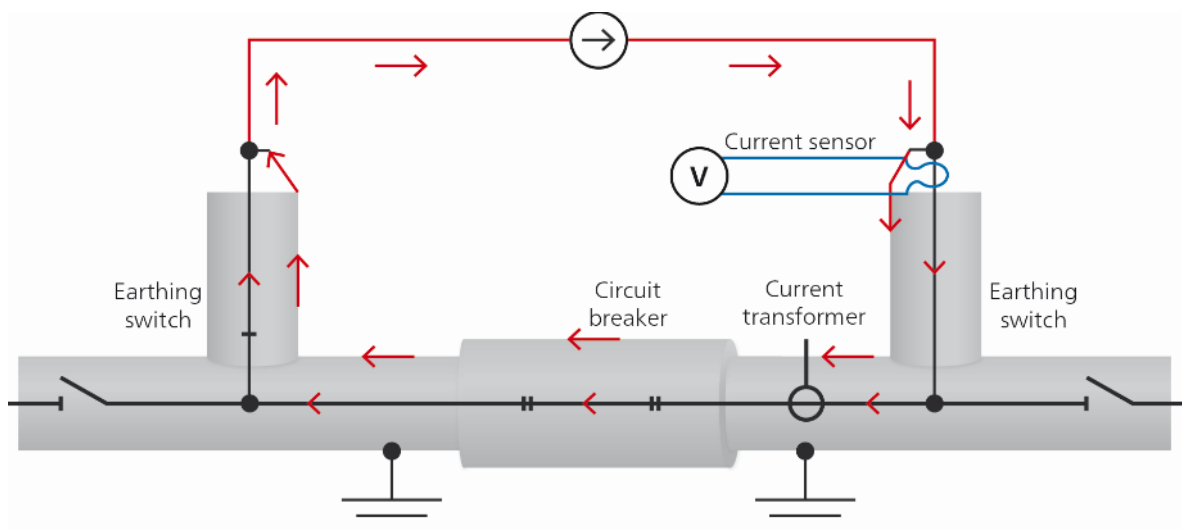
Figure 6: Rogowski coil (current sensor) through earthing switch shunt on a GIS grounded on both sides
