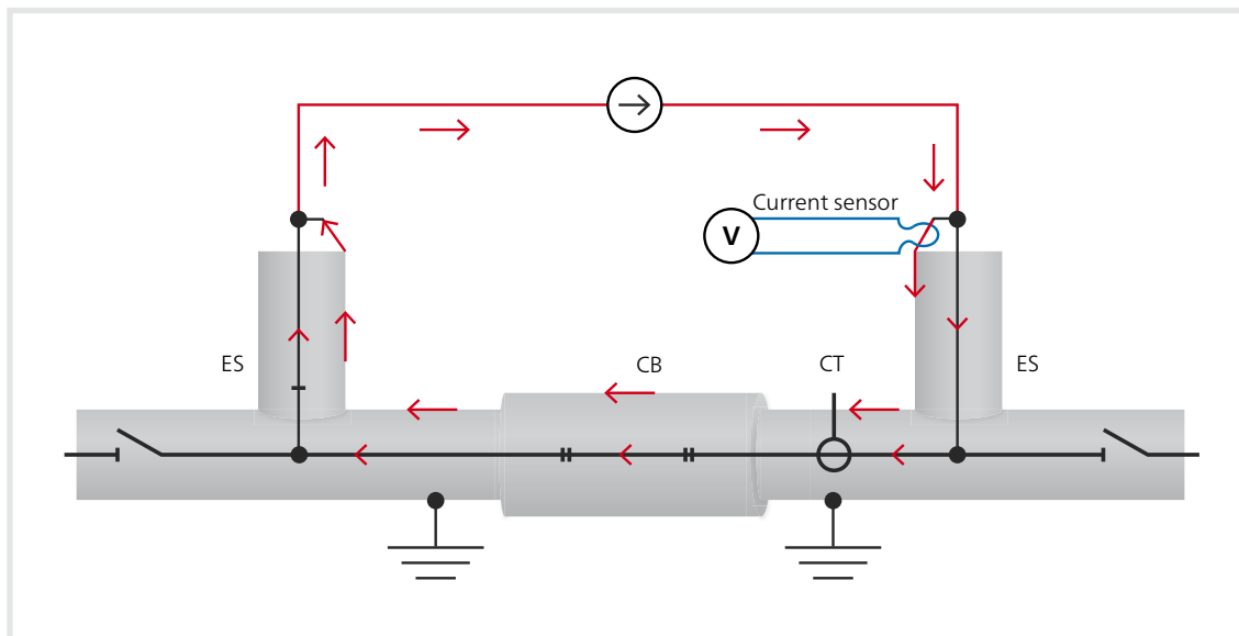
Inductive measurement of the current change using the parallel ground connection for measuring the operating times of a GIS with grounding on both sides.
