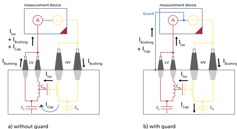
Figure 3: CHL measurement on a 2 winding transformer without and with guard
