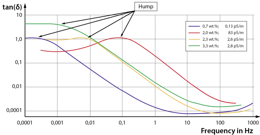
Figure 4: Broadband dielectric response of four different power transformers at 20°C
