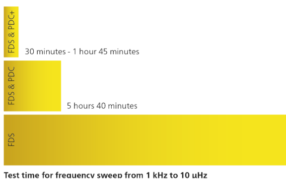
Figure 7: Test time for a frequency sweep from 1 kHz to 10 \mu Hz
