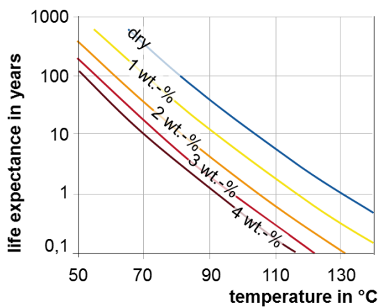
Figure 2 Dependency of life expectancy on moisture content and temperature [1]
