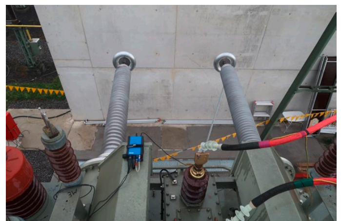
Figure 2 Setup for PD measurements on phases 1U and 1V
