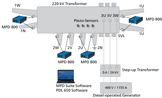
Figure 3 Setup for the PD measurements
