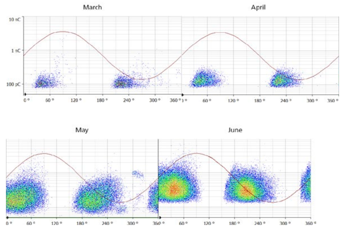
Figure 14 3PARD filtered PRPD pattern and development of the pattern obtained a Phase 1V
