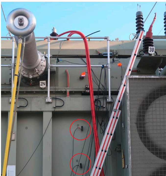
Figure 8 Installation of piezo sensors
