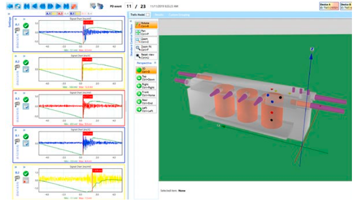
Figure 9 Acoustic signals of piezo sensors
