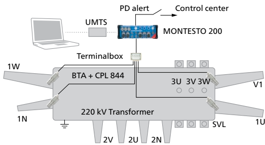
Figure 11 Complete setup of the PD monitoring and trending system
