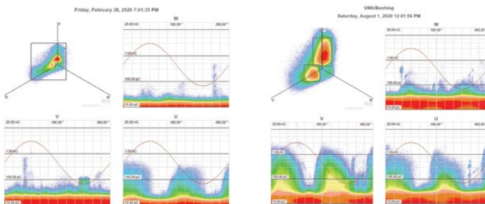
Figure 13 Development of PD activity over a period of 5 months, logarithmic view
