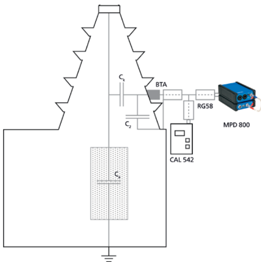
Figure 4 Artificial impulse injected directly at the bushing tap
