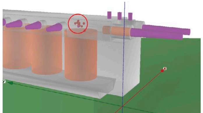
Figure 10 Location of PD at the high-voltage exit of phase 1U
