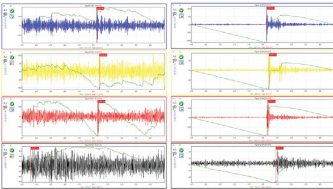
Figure 7 Acoustic signals without averaging (left) and the averaging of 100 events (right) using the electrical signal as trigger
