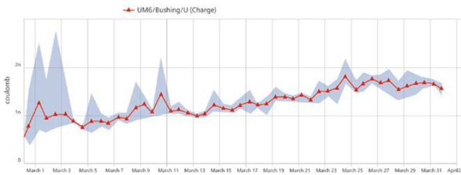
Figure 12 Increasing PD trend on Phase 1U
