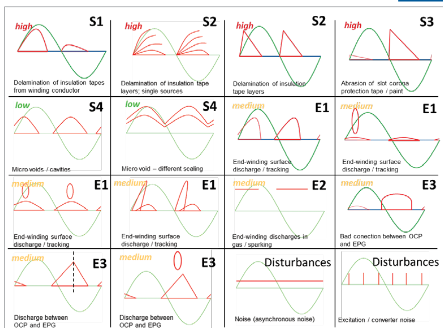
Classification of PD patterns for rotating machines
