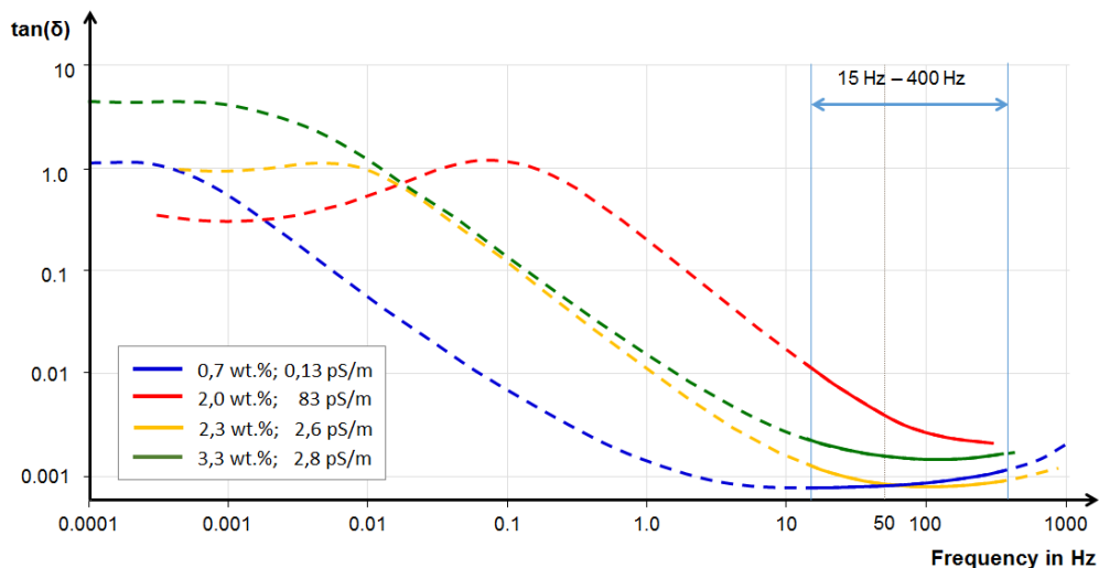
Figure 6. Broadband dielectric response of 4 different power transformers at 20°C. (Frequency in Hz)
