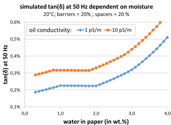
Figure 2. Dielectric properties of a power transformer oil-paper High- to the Low-voltage winding insulation (CHL)
