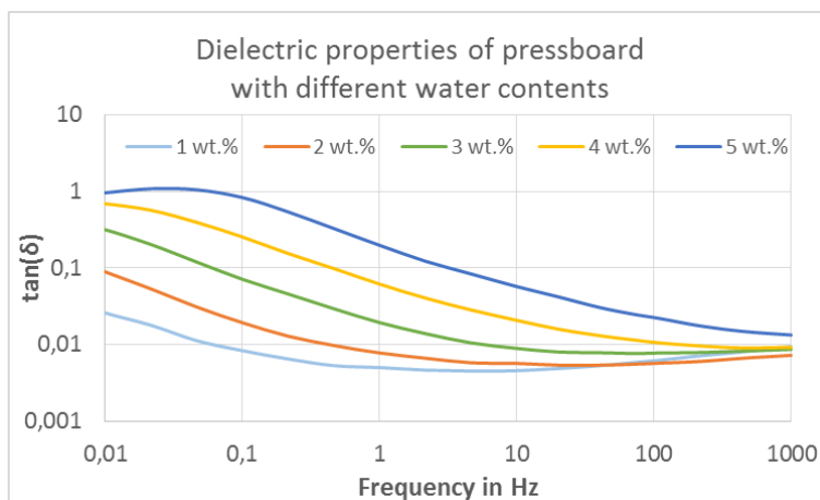
Figure 1. Dielectric properties of oil impregnated pressboard at different water contents at 20°C. (Dielectric properties of pressboard with different water contents Frequency in Hz, 1 wt. %)
