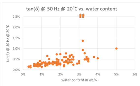
Figure 5. Ratio of \tan(\delta) at 50 Hz and 20 °C to the water content in the cellulose at over 100 power transformers, assessed via broadband dielectric measurement using the OMICRON DIRANA test system. ( \tan(\delta) @ 50 Hz @ 20 °C vs. water content; water content in wt. %)
