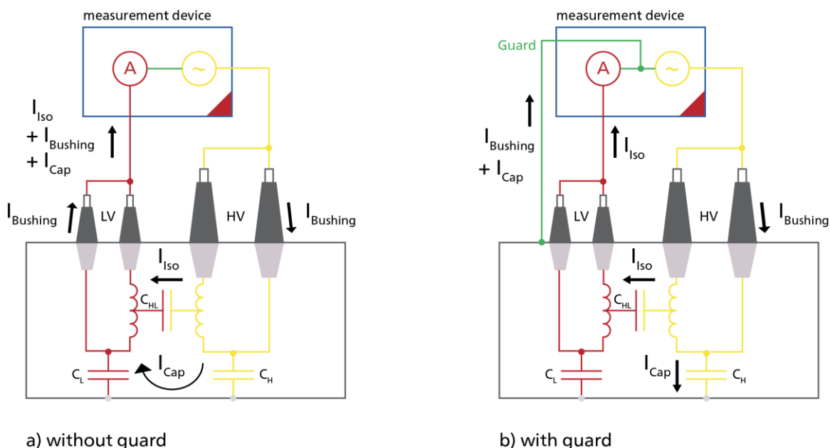
Figure 4. CHL measurement on a two-winding transformer without and with guard (measurement device; ISO; Bushing; Cap; without guard; Guard; with guard)
