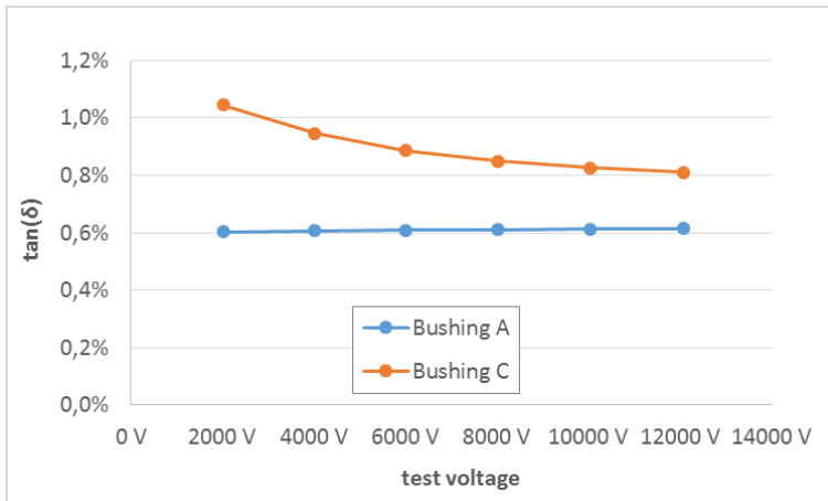
Figure 9. Tan( \delta ) measurements of two 123 kV RBP bushings of the same type at different voltages with contact problems at the measurement tap of bushing C (data from [8]) (Bushing A, Bushing C; test voltage)
