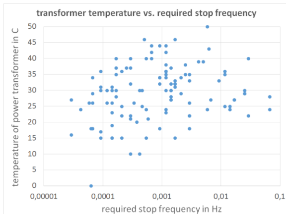
Figure 7. Required stop frequency, depending on the transformer temperature in a survey including over 100 power transformers (transformer temperature vs. required stop frequency; temperature of power transformer in C; required stop frequency in Hz)
