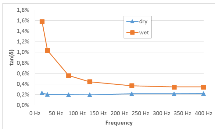
Figure 8. Frequency variable \tan(\delta) of a dry and a wet 33 kV OIP bushing at 30°C (data from [8]) (dry; wet)
