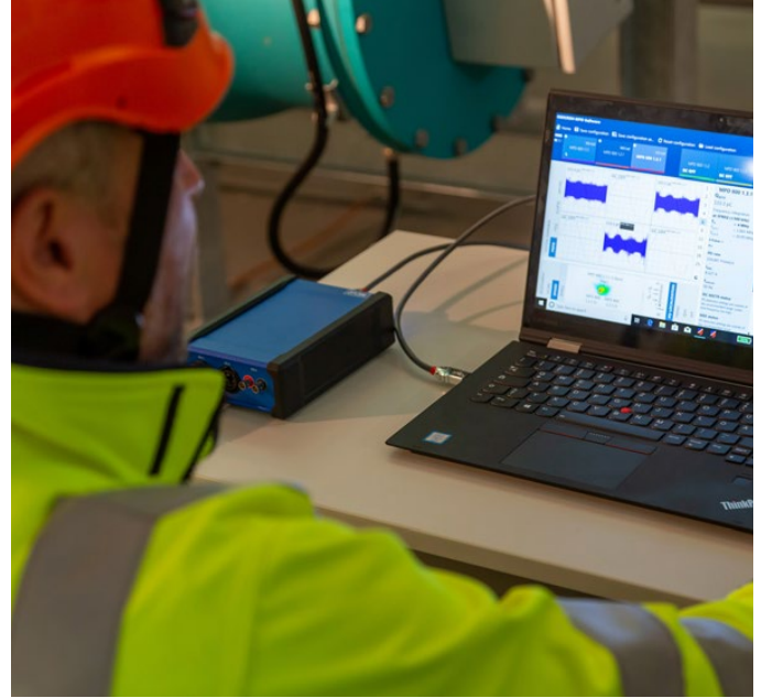
PD measurements being performed with the MPD 800 on cable system terminations.
