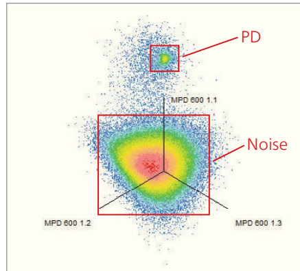
3-Phase Amplitude Relation Diagram (3PARD)
