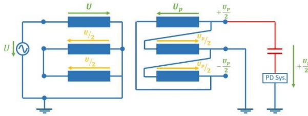
Figure 4 Test setup of a single-phase induced voltage test for a Dyn transformer.
