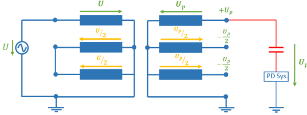
Figure 3 Test setup of a single-phase induced voltage test for a YNyn0 transformer.
