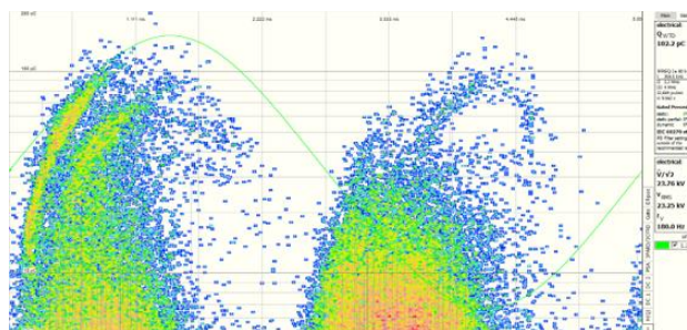
Figure 12 PRPD U-phase of the transformer, recorded during the induced voltage test.
