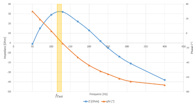
Figure 7 Frequency dependence of the test circuit impedance, amplitude (blue) and phase shift (orange).
