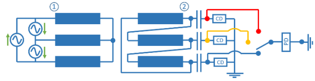
Figure 1 PD measuring configuration according to IEC 60073-11[3].
