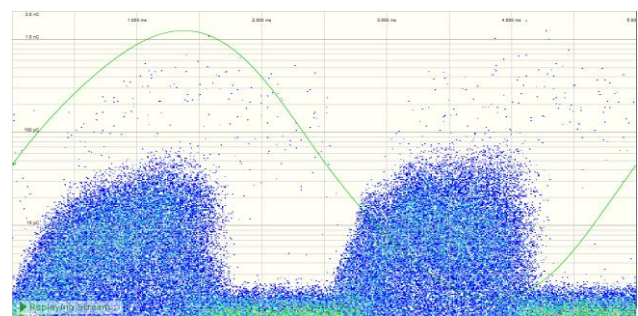
Figure 8 Surface discharges on the HV winding.
