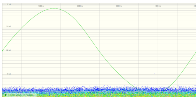
Figure 10 PRPD free of partial discharge after swapping the coupling capacitor and ground.
