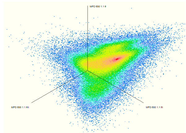
Figure 5 3CFRD of a transformer with multiple PD sources
