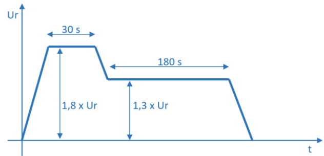
Figure 2 PD measurement test cycle according to IEC 60073-11 [3].
