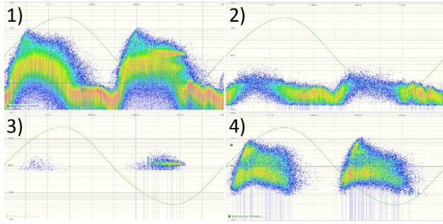
Figure 6 1) Complete PRPD, 2) Background noise, 3) Corona discharge, 4) Advanced surface discharge, after separation using 3CFRD.
