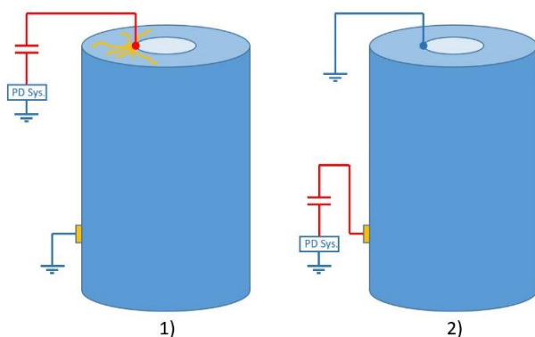
Figure 9 1) Connection of the coupling capacitor at the top of the winding, surface discharges 2) Coupling capacitor and ground swapped, free of PD.
