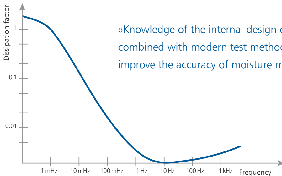
Dielectric response measurement graph
