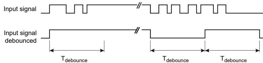
Figure 2-3: Signal curve, debounce input signals
