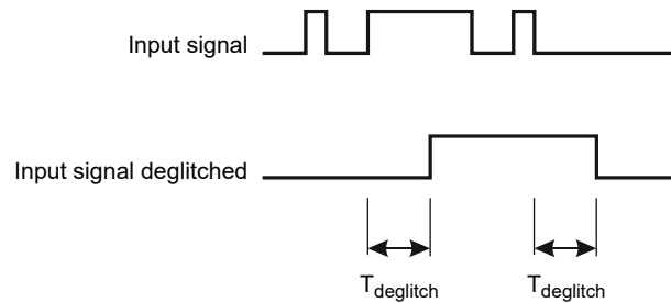
Figure 2-2: Signal curve, deglitching input signals
