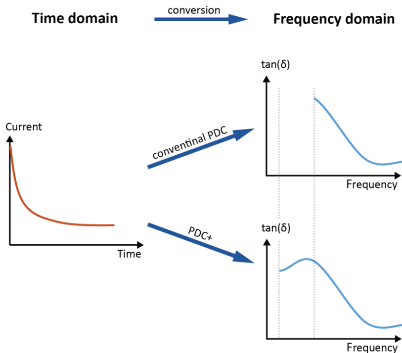
Figure 6: Conversion from time to frequency domain for conventional PDC and PDC+
