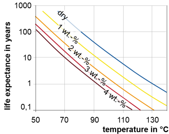
Figure 2 Dependency of life expectancy on moisture content and temperature [1]
