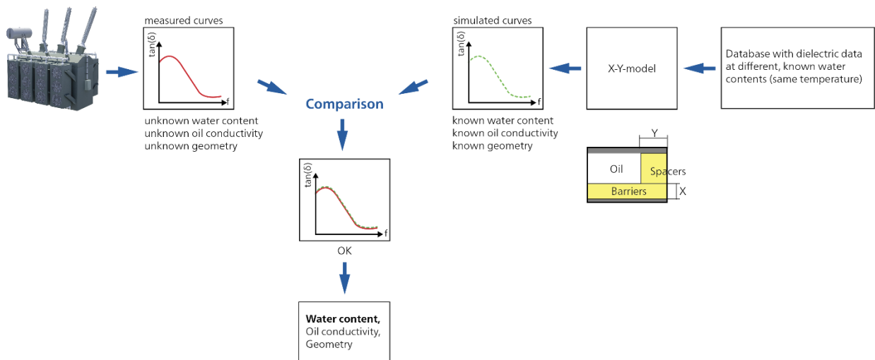
Figure 5: Principle of the water content assessment of power transformers
