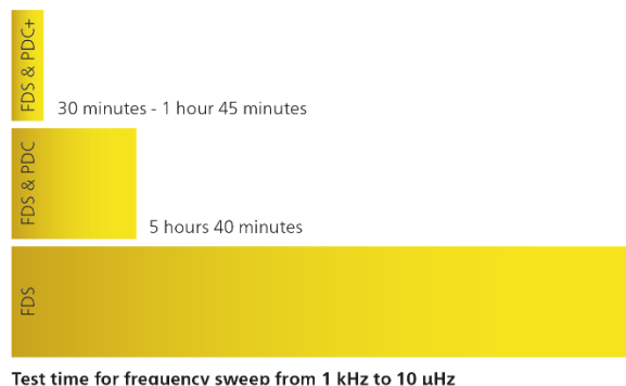
Figure 7: Test time for a frequency sweep from 1 kHz to 10 \mu Hz
